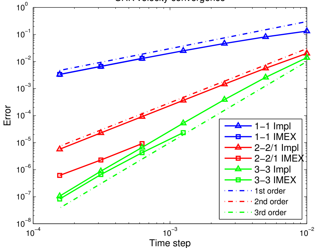
SRK velocity convergence
