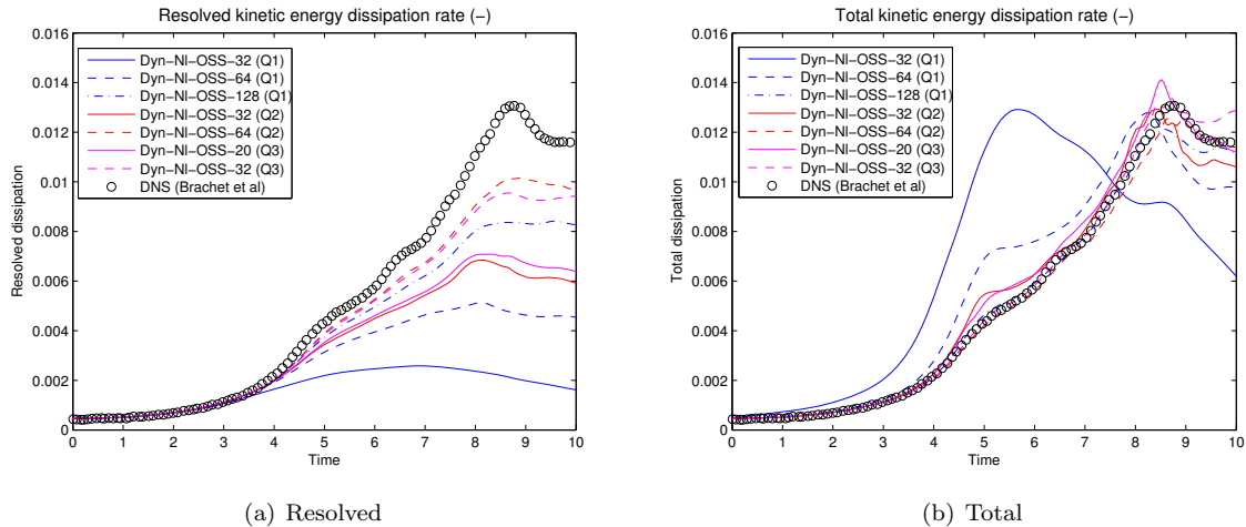
Figure 11: Dissipation rate evolution for the h - p refinement cases.
