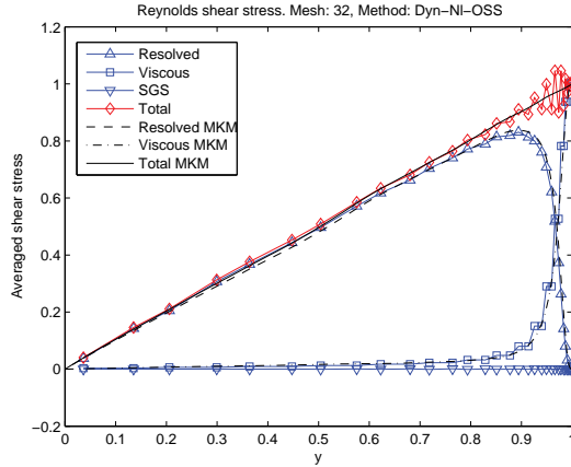
Figure 15: Reynolds stress of the Dyn-NI-OSS case.
