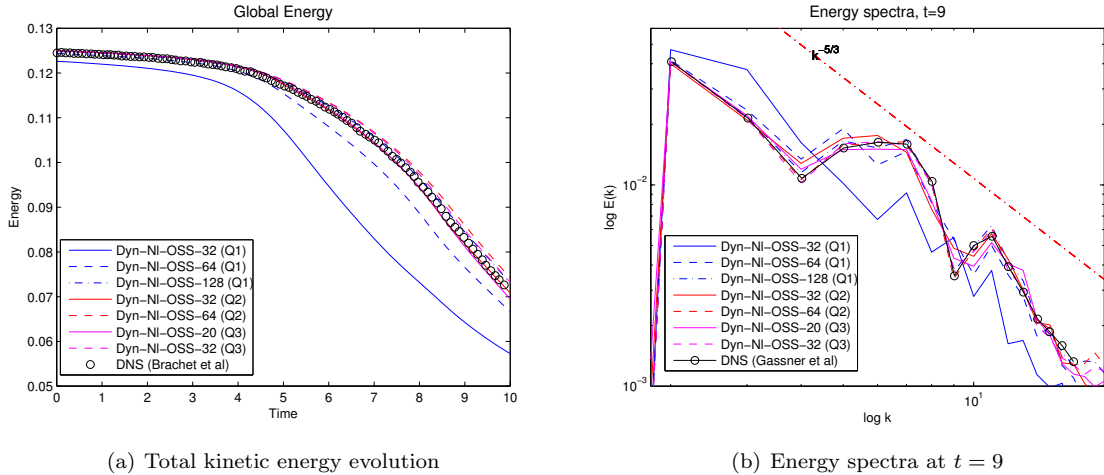
(a) Total kinetic energy evolution
