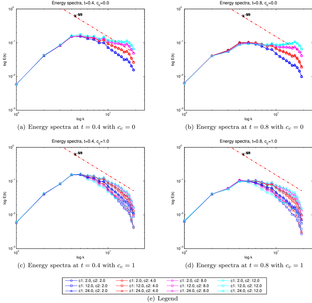
Figure 16: Comparison of energy spectra for different c_1 , c_2 and c_c in the DHIT test.
