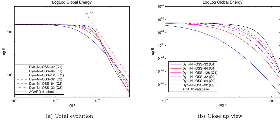
Figure 7: Total kinetic energy evolution.
