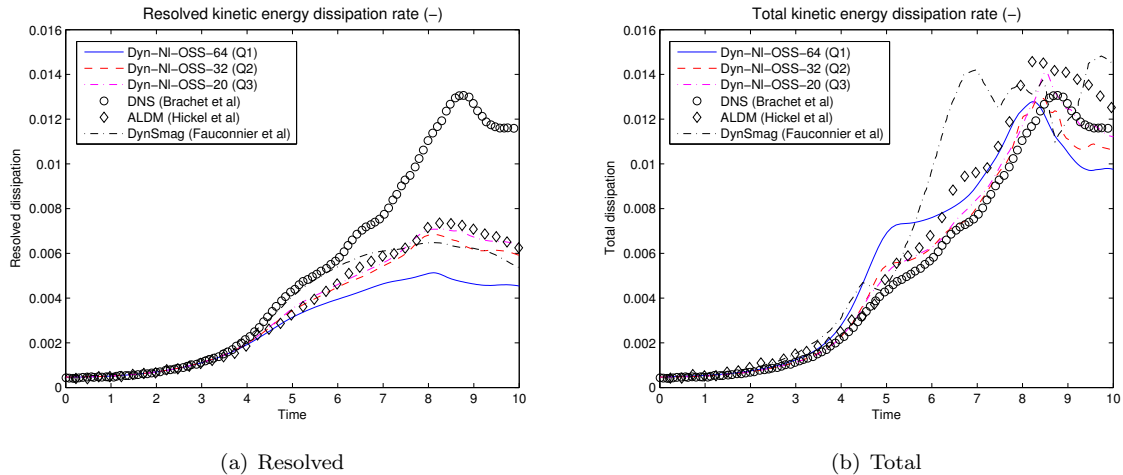
Figure 12: Dissipation rate evolution compared to the dynamic Smagorinsky [29] and ALDM models [40].
