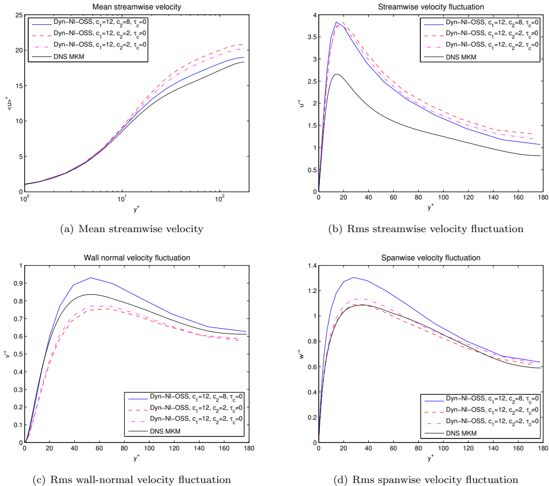
Figure 17: Comparison of mean streamwise velocity and rms velocity fluctuations for Re_\tau = 180 case using a 32^3 Q1 mesh.
