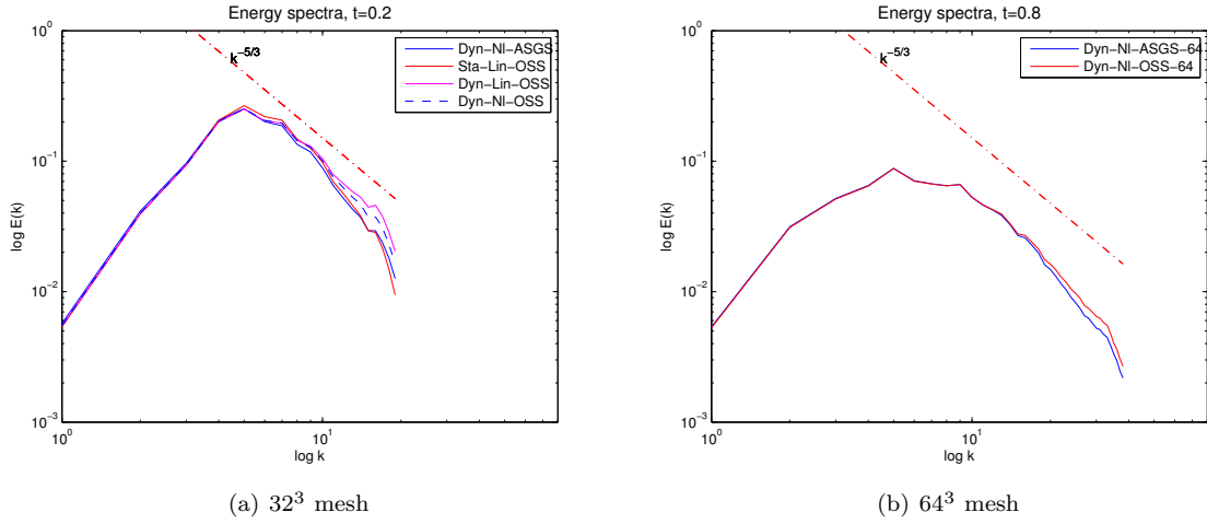
Figure 6: Energy spectra at t = 0.2 ( 32^3 mesh) and t = 0.8 ( 64^3 mesh).
