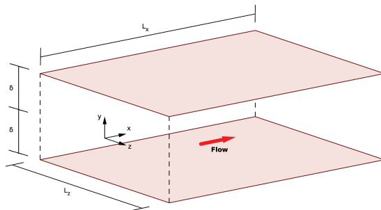
Figure 13: Channel computational domain.
