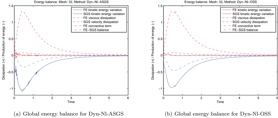
Figure 3: Global energy balance using skew-symmetric convective term type 2 .
