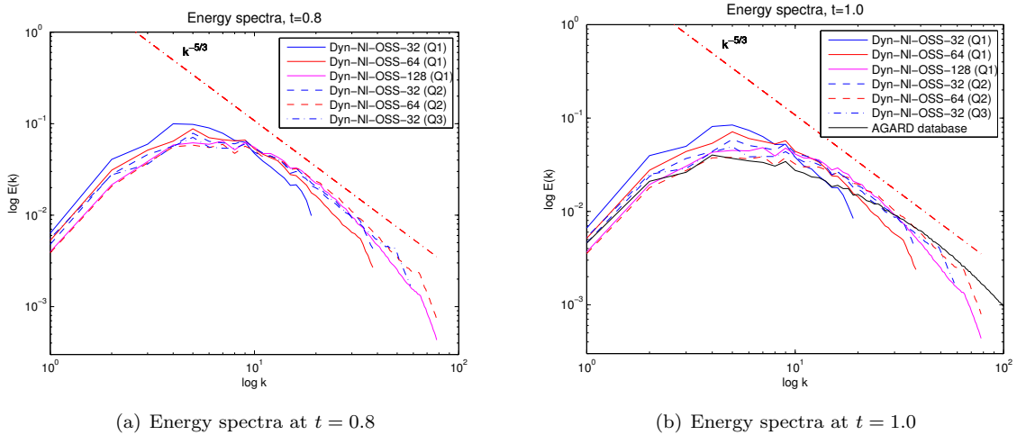
Figure 8: Energy spectra at t = 0.8 and t = 1.0 for the h - p refinement defined in Table 2.
