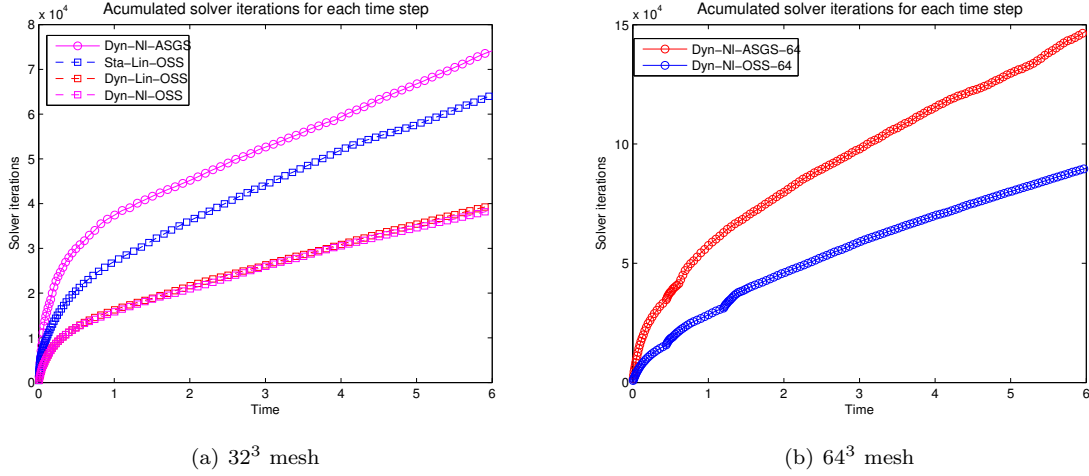
Figure 4: Accumulated solver iterations.
