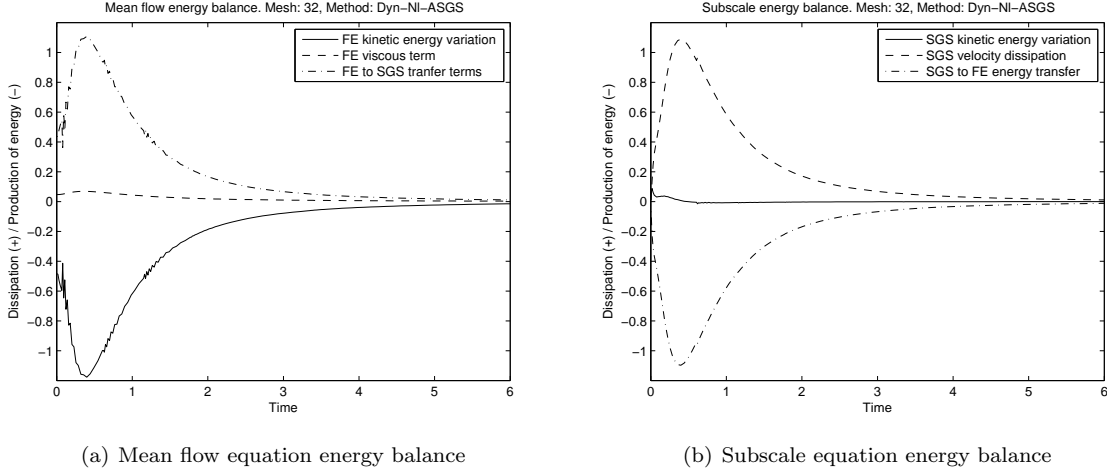
Figure 1: Mean flow and subscale energy balances for the Dyn-NI-ASGS method.
