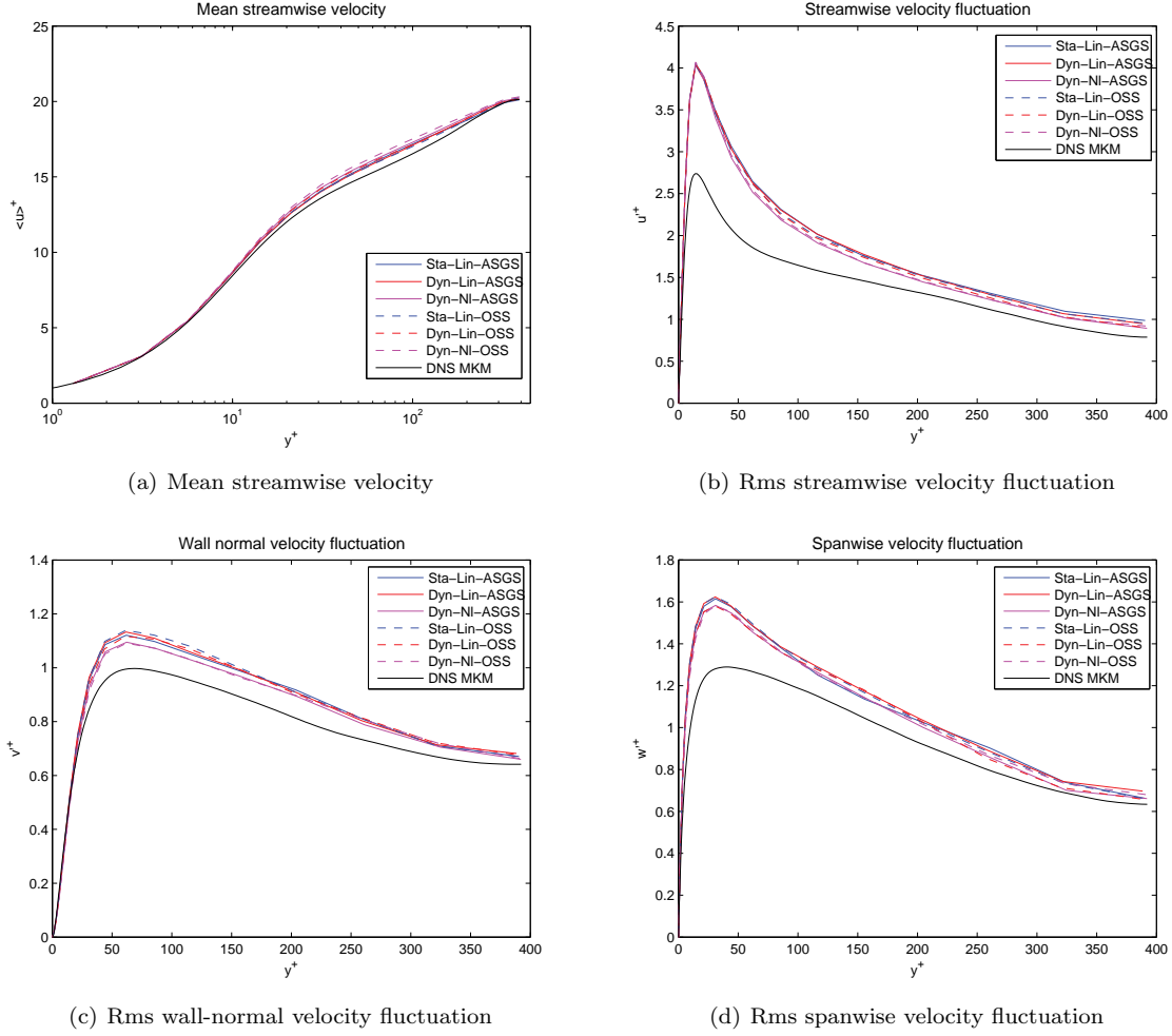
Figure 14: Mean streamwise velocity and rms velocity fluctuations for Re_\tau = 395 case using a 32^3 Q_1 mesh.
