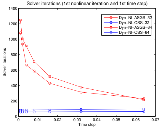
Figure 18: Solver iterations at the first time step for DHIT test.
