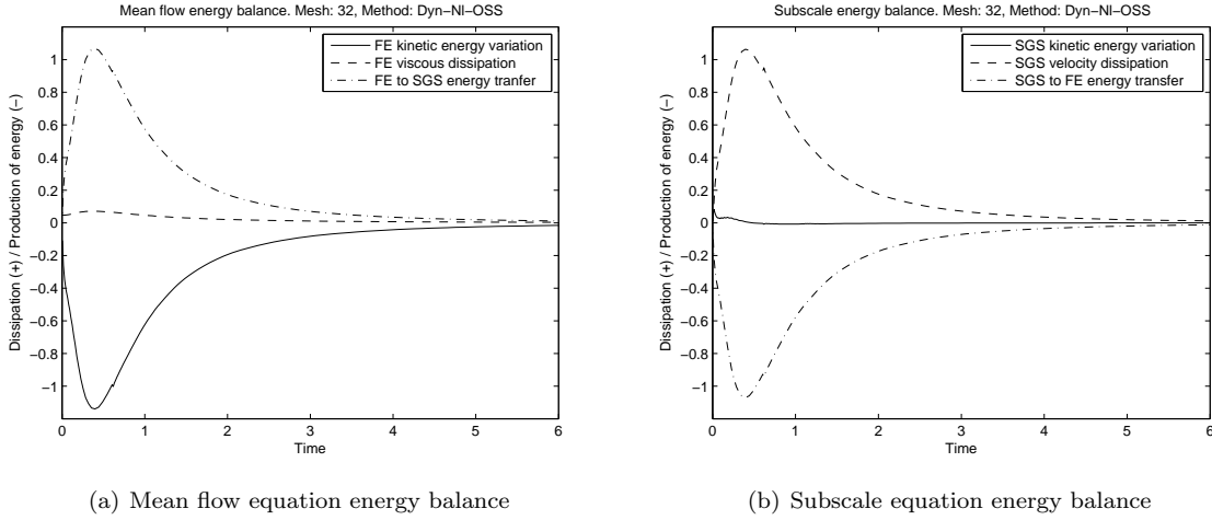
Figure 2: Mean flow and subscale energy balances the Dyn-NI-OSS method.
