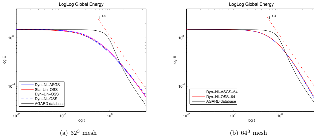
Figure 5: Total energy evolution for the 32^3 and 64^3 elements meshes with the scaled initial condition.
